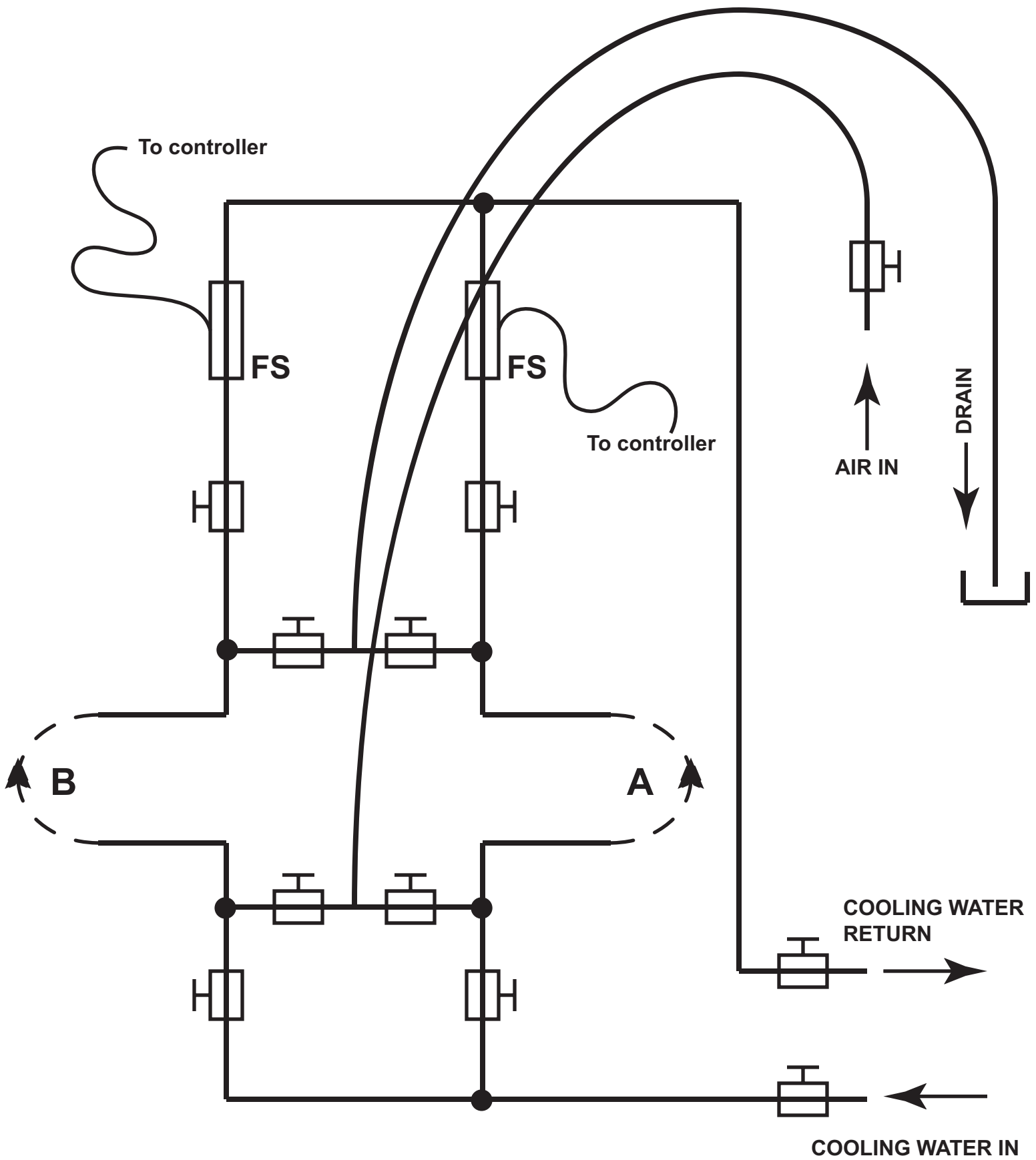
Piston cylinder cooling system
